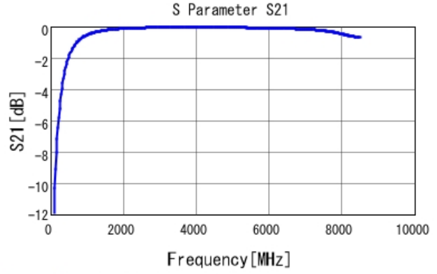
GRM1555C1H4R2CA01 S21 DCOV, 25degC
