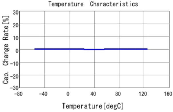
GRM1555C1H4R2CA01 C-Temp. capchange, DCOV, AC1Vrms
