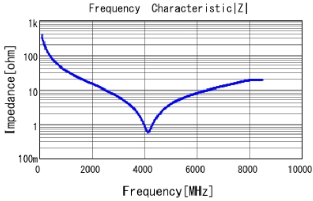
GRM1555C1H4R2CA01 |Z| DCOV, 25degC
