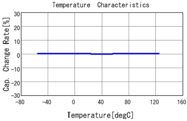
GRM1555C1H4R2WA01 C-Temp. capchange, DCOV, AC1Vrms
