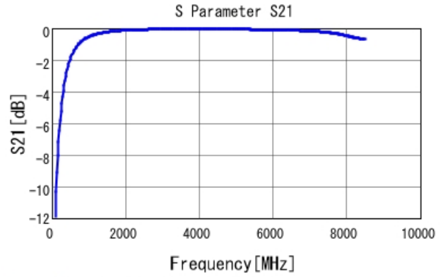
GRM1555C1H4R2WA01 S21 DCOV, 25degC
