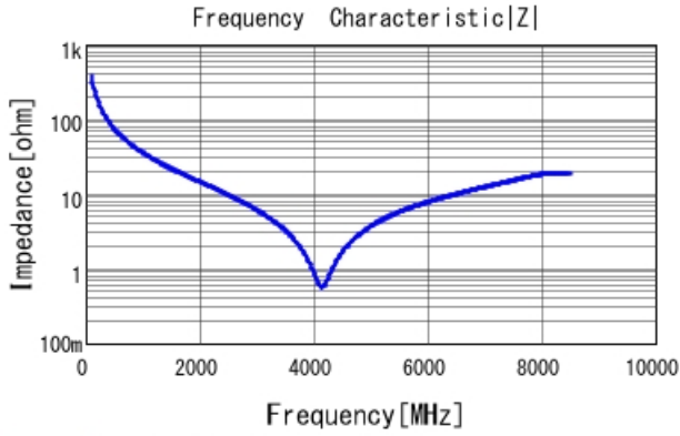
GRM1555C1H4R2WA01 |Z| DCOV, 25degC
