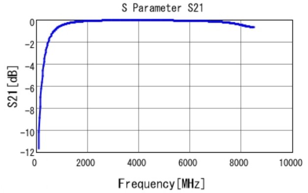
GRM1555C1H4R3WA01 S21 DCOV, 25degC
