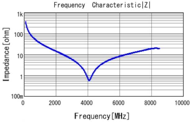
GRM1555C1H4R3WA01 |Z| DCOV, 25degC
