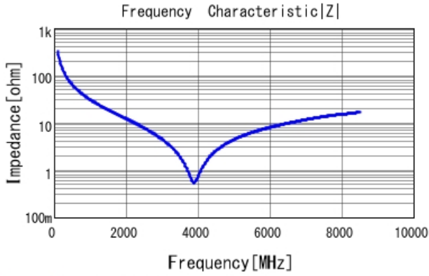
GRM1555C1H4R8BA01 |Z| DCOV, 25degC
