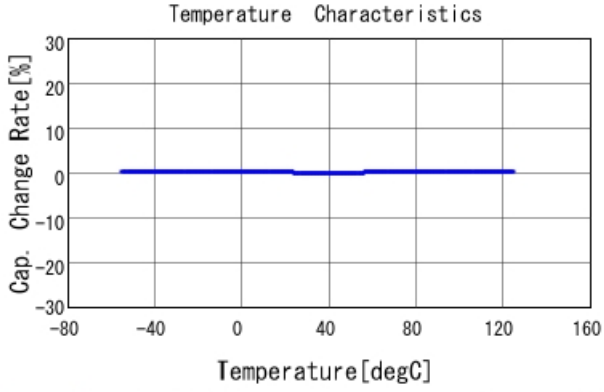
GRM1555C1H4R8BA01 C-Temp. capchange, DCOV, AC1Vrms
