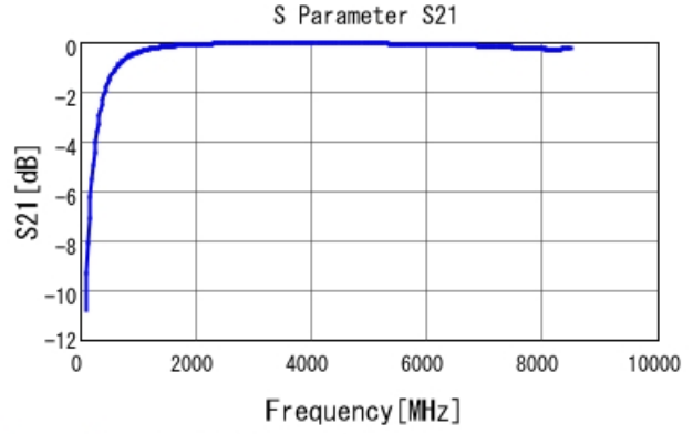
GRM1555C1H4R8BA01 S21 DCOV, 25degC
