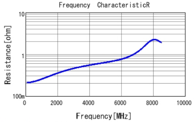
GRM1555C1H4R8BA01 R DCOV, 25degC
