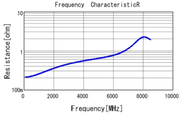
GRM1555C1H4R9WA01 R DCOV, 25degC
