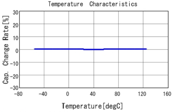
GRM1555C1H4R9WA01 C-Temp. capchange, DCOV, AC1Vrms
