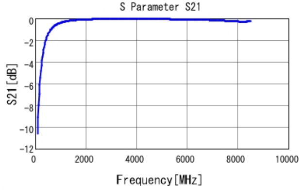
GRM1555C1H4R9WA01 S21 DCOV, 25degC
