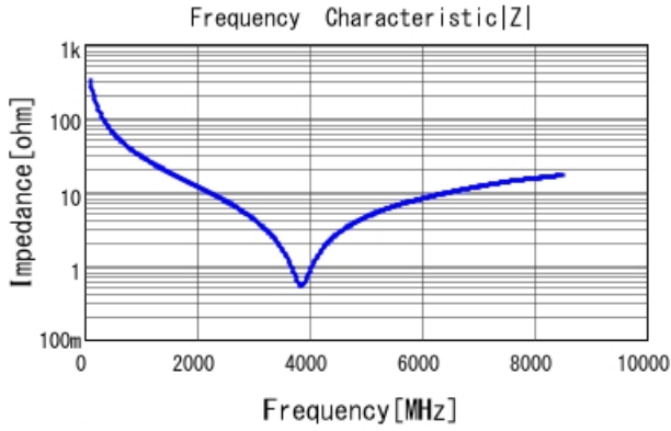
GRM1555C1H4R9WA01 |Z| DCOV, 25degC
