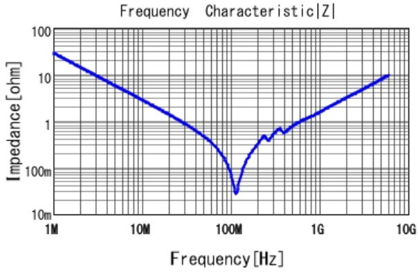
GRM1555C1H562GE01 |Z| DCOV, 25degC
