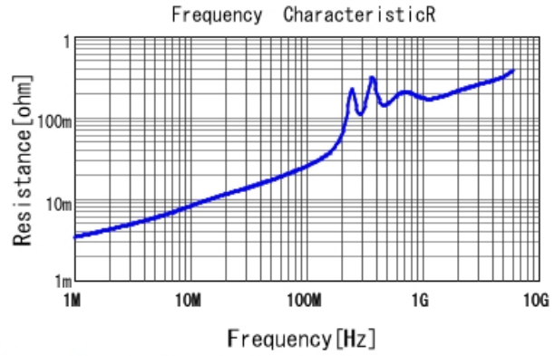
GRM1555C1H562GE01 R DCOV, 25degC
