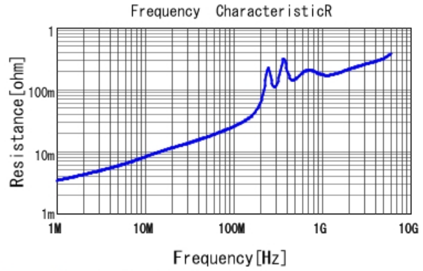
GRM1555C1H562JE01 R DCOV, 25degC
