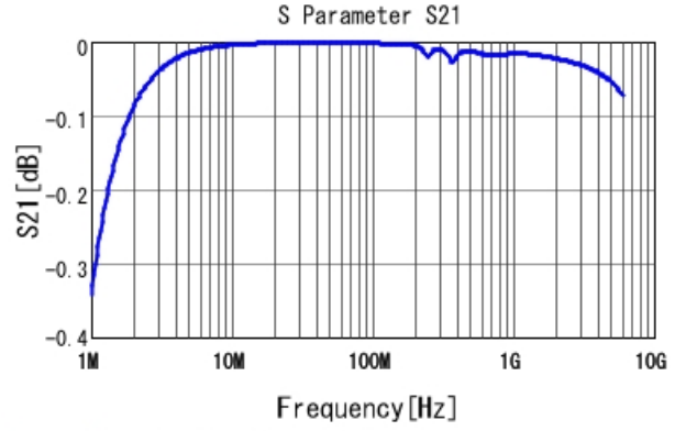
GRM1555C1H562JE01 S21 DCOV, 25degC
