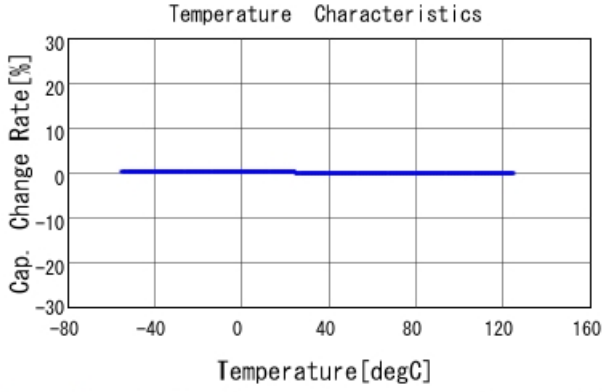
GRM1555C1H562JE01 C-Temp. capchange, DCOV, AC1Vrms
