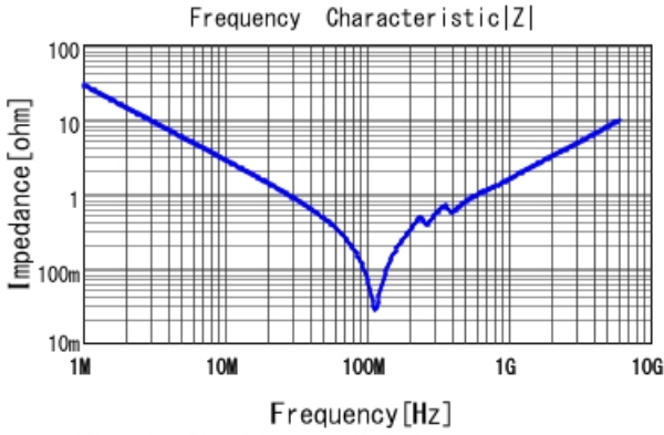
GRM1555C1H562JE01 |Z| DCOV, 25degC
