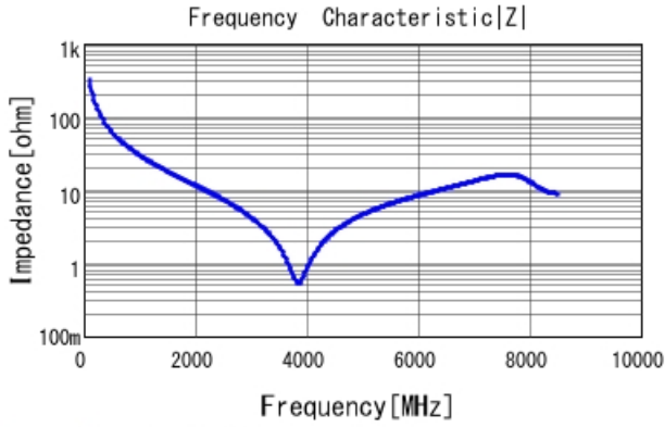
GRM1555C1H5R0BA01 |Z| DCOV, 25degC
