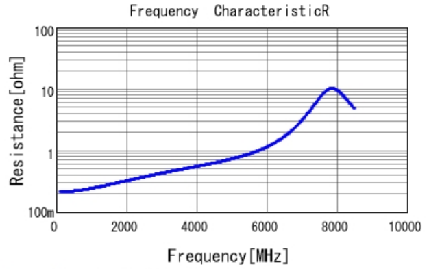
GRM1555C1H5R0BA01 R DCOV, 25degC
