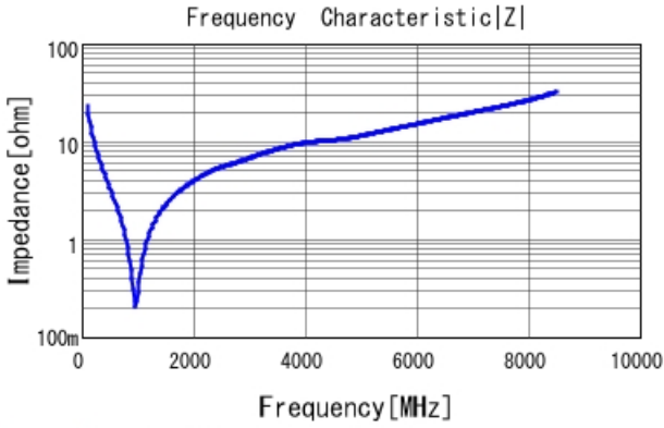
GRM1555C1H680GA01 |Z| DCOV, 25degC
