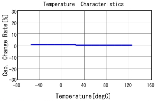
GRM1555C1H680GA01 C-Temp. capchange, DCOV, AC1Vrms
