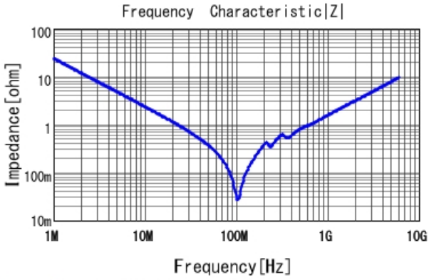
GRM1555C1H682JE01 |Z| DCOV, 25degC
