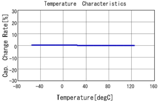
GRM1555C1H682JE01 C-Temp. capchange, DCOV, AC1Vrms
