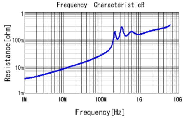
GRM1555C1H682JE01 R DCOV, 25degC
