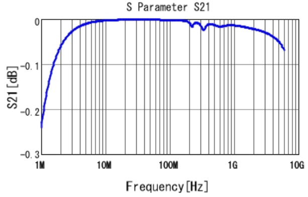
GRM1555C1H682JE01 S21 DCOV, 25degC
