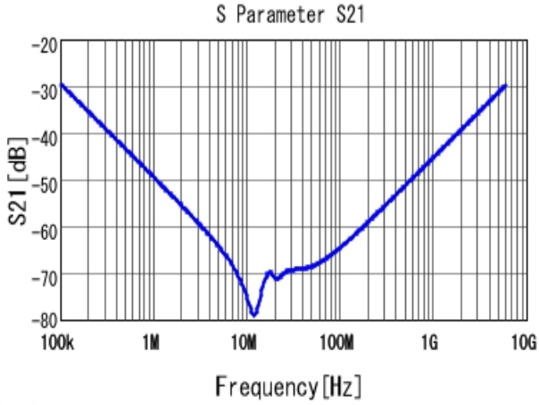
■ NFM21PC225B0J3 S21 DC0V, 25degC, Feedthrough
