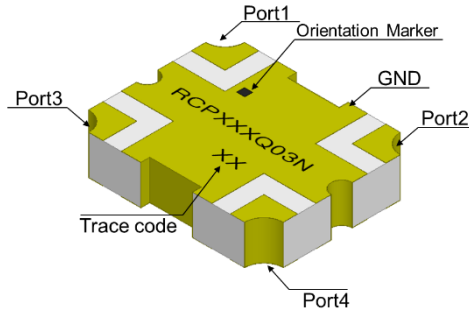
Figure 1. RCP1850Q03N (Top View)
