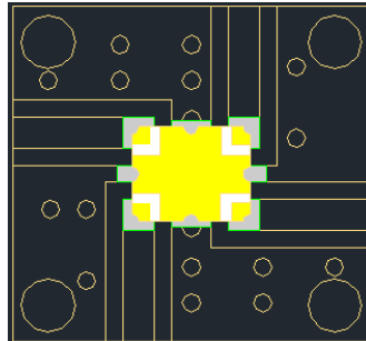
Figure 11. Placing the RCP2150Q03 on the 9 Points of the PCB Surface
