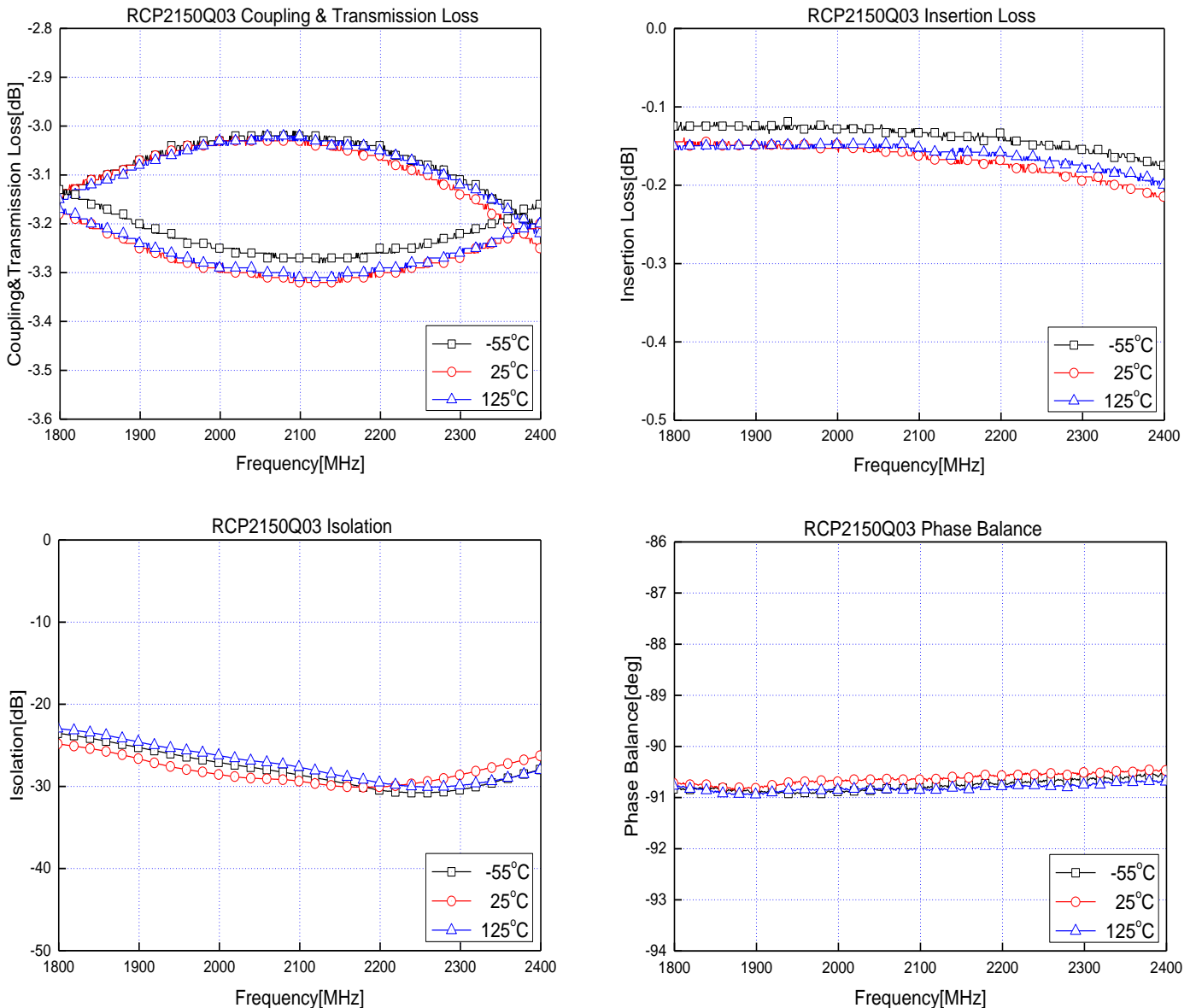
Figure 4. Test Plots of Coupling and Transmission Loss, Insertion Loss, Isolation, and Phase Balance (-55 °C, 25 °C, and 125 °C)
