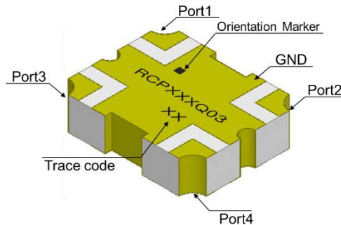
Figure 1. RCP2300Q03 (Top View)
