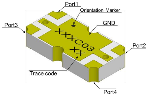
Figure 1. RCP2600C03 (Top View)
