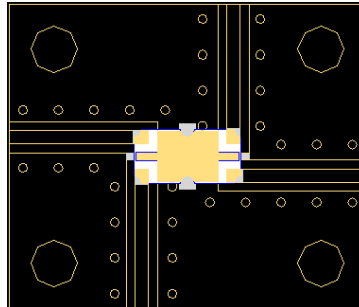
Figure 11. Placing the RCP2600C03 on the 8 Points of the PCB Surface
