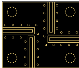
Figure 9. Cleaning the PCB Surface Where the RCP2600C03 is Soldered
