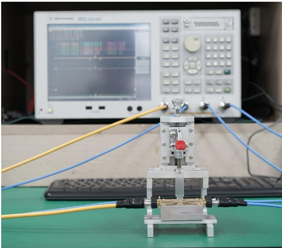
Figure 5. Test Setting to Measure the RCP3500A03 S-parameters
