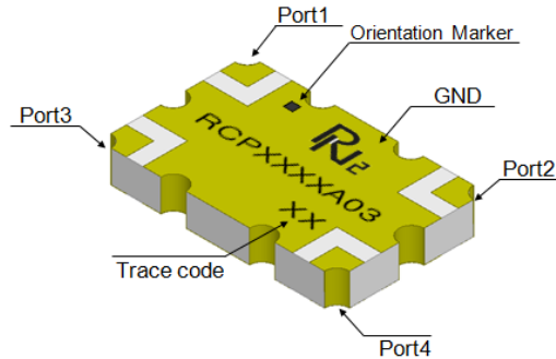
Figure 1. RCP3500A03 (Top View)
